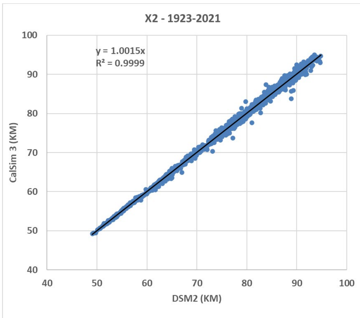
Figure 4A-6-4. X2 comparison for CalSim3 (ANN) vs DSM2
