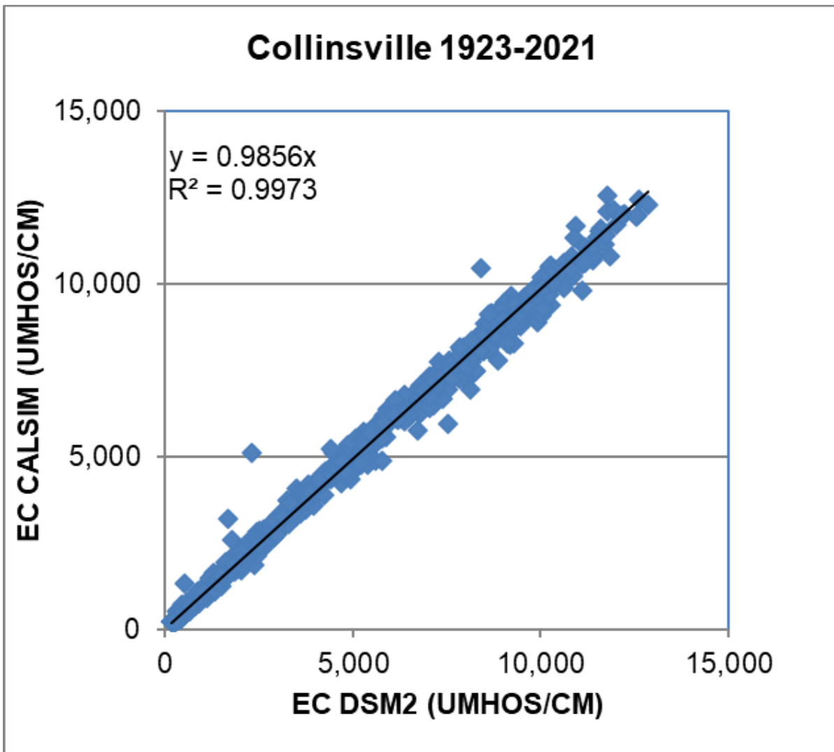
Figure 4A-6-3. Collinsville EC comparison for CalSim3 (ANN) vs DSM2
