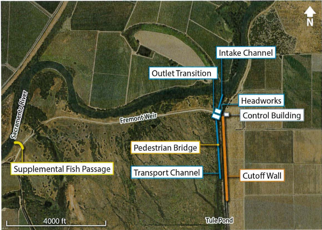
Figure 2. Alternative 1 components near the Fremont Weir
