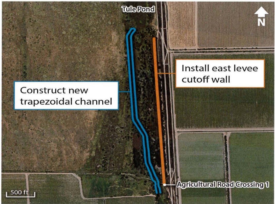
Figure 4. Downstream improvements near Agricultural Road Crossing 1
