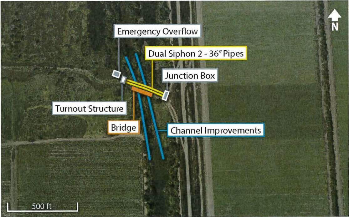
Figure 3. Improvements at Agricultural Road Crossing 1
