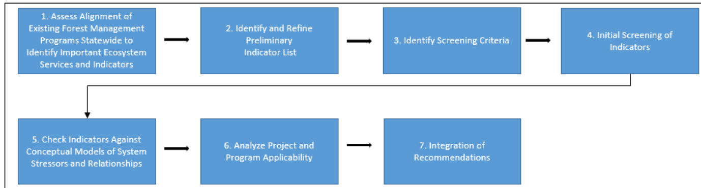
Fig. 10: Summary of suggested seven-step approach to selecting ecological performance measures. Adaptation of Baldera et al. 2018.
